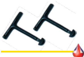
D-End Light Duty Manhole Cover Keys Malleable iron. Tee handle. D-shaped end. (w25 x 13 x 8mm).
