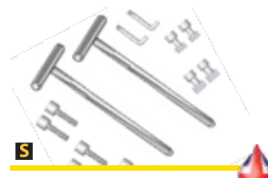
Cover Lifting Set Supplied with 2 lifting keys with 6 Pairs of interchangeable tips : T-shaped 35x15x5mm & 25x12x5mm. Threaded M8 M10 & M12 Tips and 10mm Hooked Tips.
