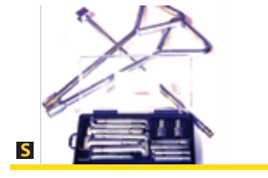
Cover Lifting Set Manhole Cover lifting set with carbon steel zinc plated interchangeable tips. Includes: 2 x 440mm Handles, interchangeable 33mm rectangular Tips, 22mm rectangular Tips, 10mm Side Entry tips, M10 Screw Tips, M12 Screw Tips, M16 Screw Adaptors. 1 Short Stopcock Tip, 1 Long Stopcock Tip. Tips in a small plastic box. ( Spare Nylon Tips 1021T )
